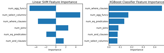
Figure 8: Importance of various SQL features for SVM and XGBoost trained for optimizing execution time.
