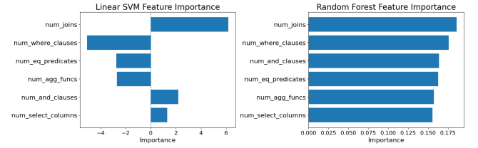
Figure 9: Importance of various SQL features for SVM and RF trained for optimizing memory.
